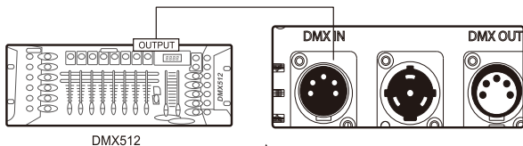
Connecting DMX to only one 300d II
