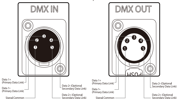
Daisy chaining multiple lights using DMX
