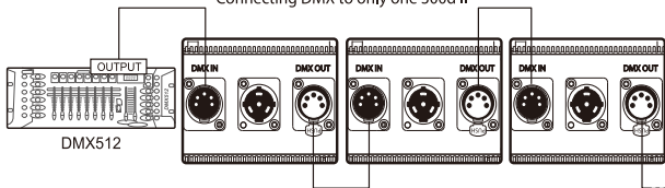
Daisy chaining multiple lights using DMX
