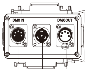
DMX IN Port
